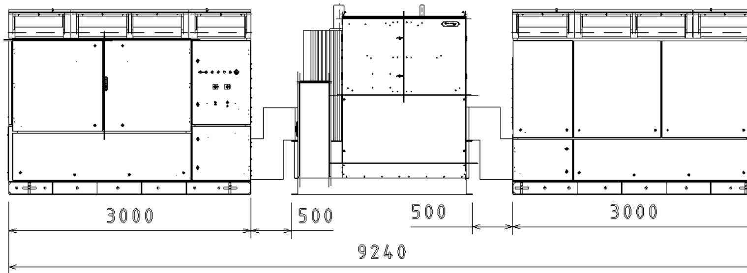
FRONT VIEW
